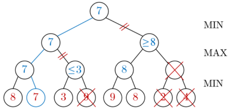
Figure 5.2: Sample alpha-beta pruning
