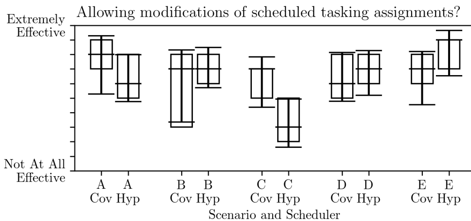
(c) Prompt 3
