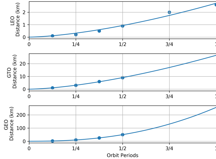
Figure 4.2: Reachability trendlines fit to reference data [84, 85]
